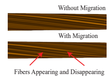
Fig. 5 Fiber migration.
