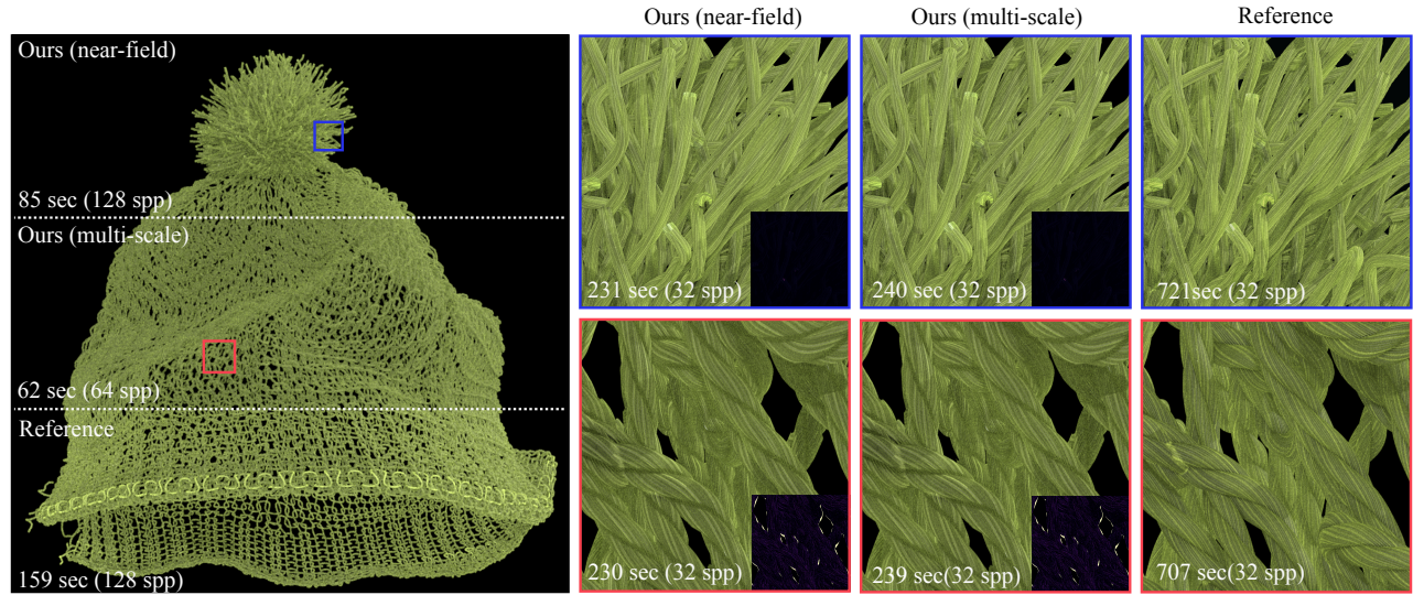
Fig. 1 In this scene we compare the rendering results of our BYSDF model (near-field and multi-scale) to the reference ply-based model for a knitted beanie, with the error map provided in the insets. Our model achieves close-matched results to the reference, both in far-away and zoomed-in views, with accurate soft shadows and geometry of plies and fibers as seen in Row I and Row II close-up, respectively. Notably, our approach achieves these results while utilizing only 20% of the memory and over 2.5 times acceleration compared to the reference under the same rendering quality (noise-level). Our multi-scale result offers additional performance gain by leveraging a level-of-detail strategy as shown in zoomed-out results. The scene has been lit using two area lights and one constant environment lighting.
