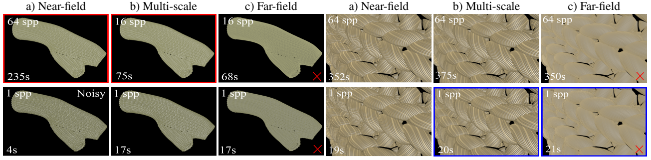
Fig. 10 Multi-scale comparison. Near-field mode captures fine details but becomes inefficient as the camera moves away. In the Multi-scale mode, we smoothly transition between near-field and far-field renderings using an adaptive scheme based on pixel coverage, yielding fewer samples. Far-field mode efficiently captures macro-scale appearance when yarn width is smaller than pixel coverage. Comparing equal quality rendering (EQ) for zoom-out (left 3 columns), our multi-scale model is around 2.4\times faster than the near-field model. Similarly, in the close-up (right 3 columns), our multi-scale model offers fiber details compared to the far-field model at a similar time. Note in the third column the yarns are still larger than one pixel so we should not use Far-field and this is for comparison only, hence marked by a red cross.
