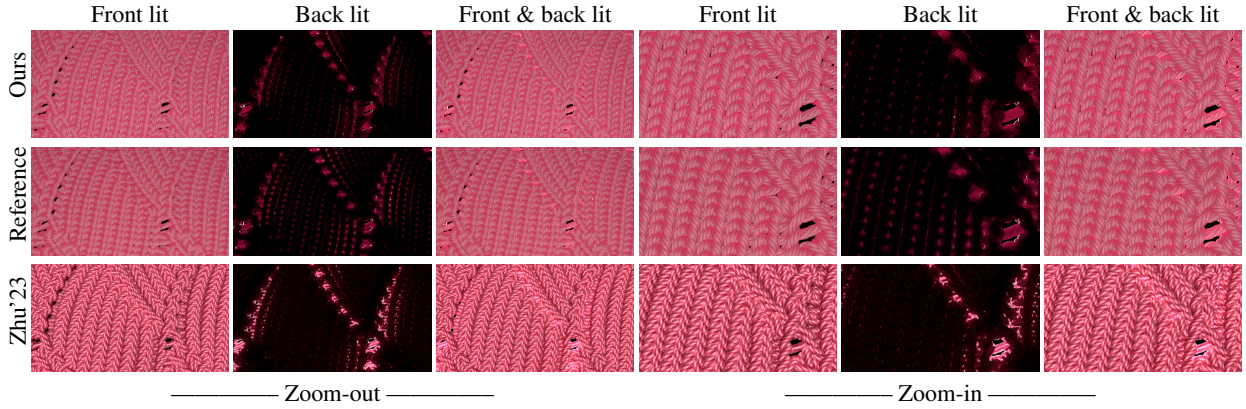
Fig. 11 Comparison with hierarchical yarn-based model Our model provides a close match to the reference ply-based model, offering faster rendering speed and reduced memory usage for this 6-ply knit sample. The performance metrics are listed in Table 1. Besides, in comparison to the hierarchical yarn-based model, ours enjoys 1.2 times faster performance as well as presenting the fiber-level detail in close-up views. Please note since their model can not accurately handle the geometric information of the multi-ply yarns, the appearance looks more rigid and lacks soft shadows with inaccurate highlights.
